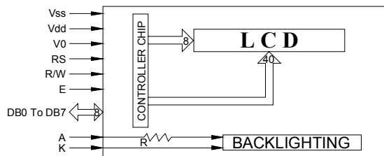
BLOCK DIAGRAM
