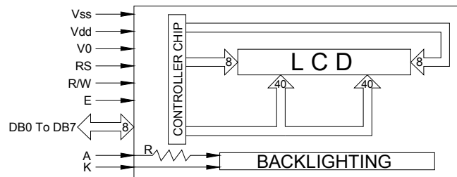
BLOCK DIAGRAM
