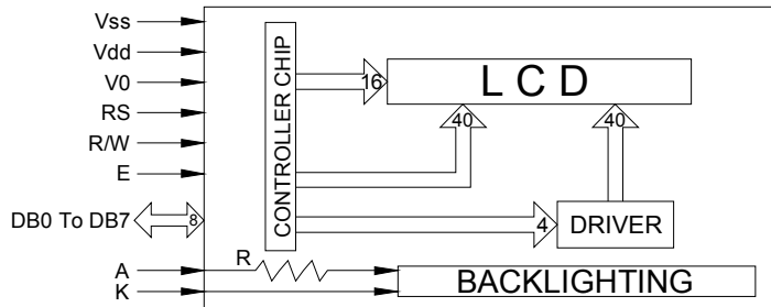
BLOCK DIAGRAM
