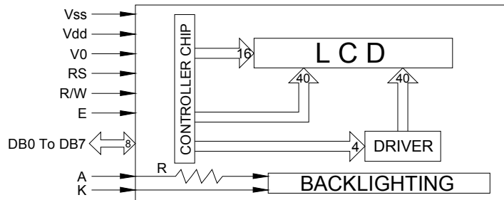
BLOCK DIAGRAM
