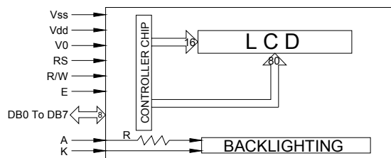
BLOCK DIAGRAM
